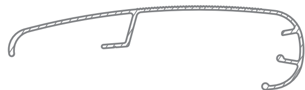
UA4474 177.6mm x 50.96mm Seating Back
