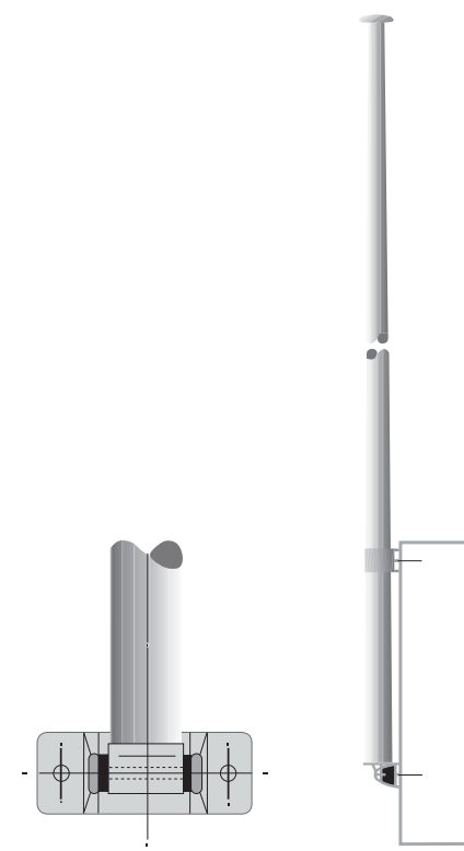
TYPE B3 Hinged parapet mounted pole for a single storey building where the pole can be laid down on the ground for servicing, replacing halyards or painting
