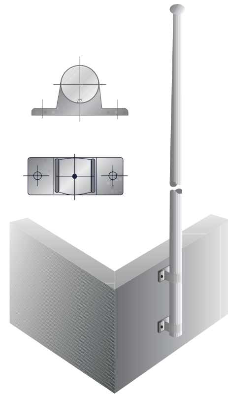
TYPE B1 Fixed parapet mounted pole
