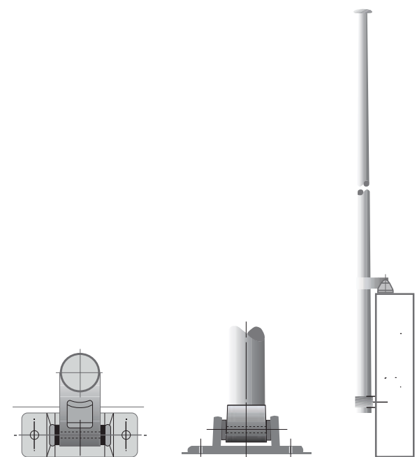
TYPE B2 Hinged parapet mounted pole designed to lay onto the roof of the building for servicing, replacing halyards or painting
