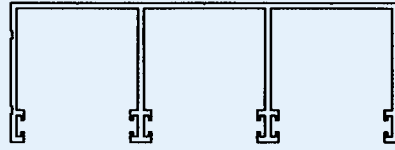
AS8096 TRIPLE TRACK HEAD
